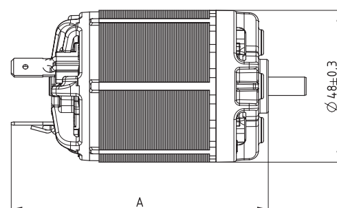
A = 70 mm (stack height 13 mm)
